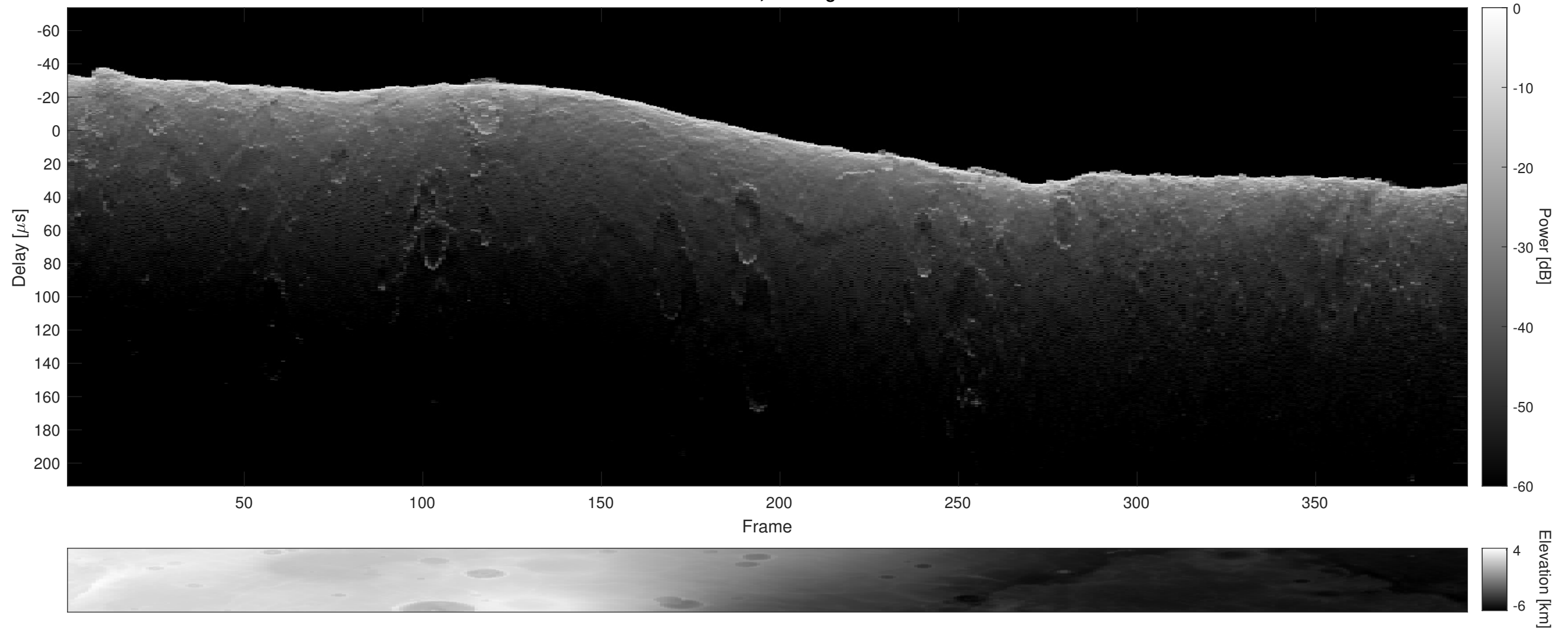
Orbit 20890, Cluttergram
