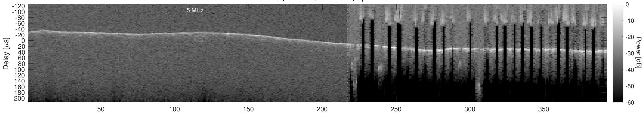
Orbit 20890, Cluttergram
