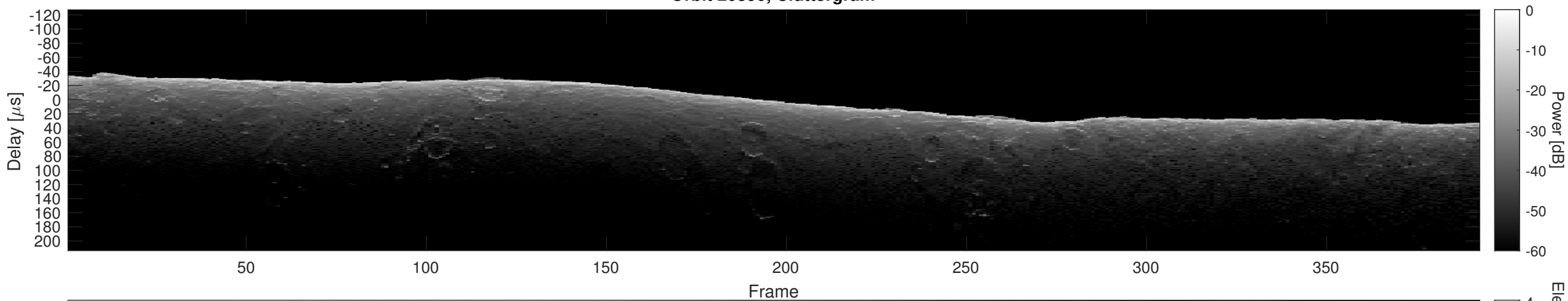
Orbit 20890, Cluttergram
