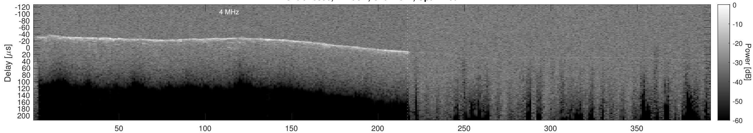
Orbit 20890, Cluttergram
