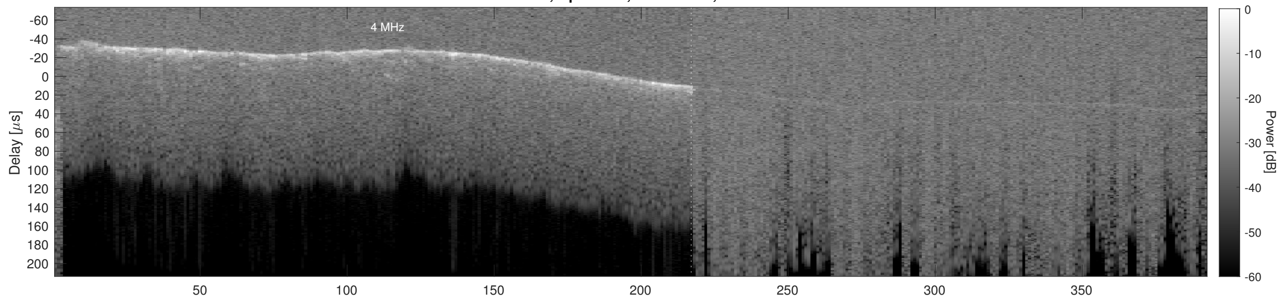
Orbit 20890, Cluttergram
