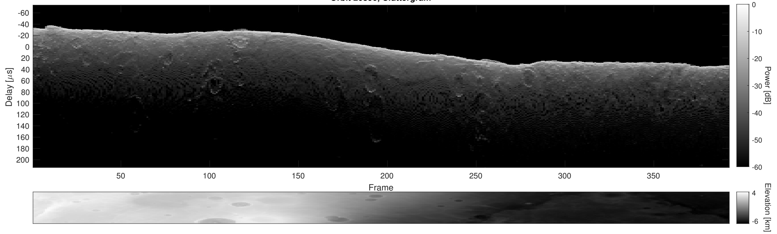
Orbit 20890, Cluttergram
