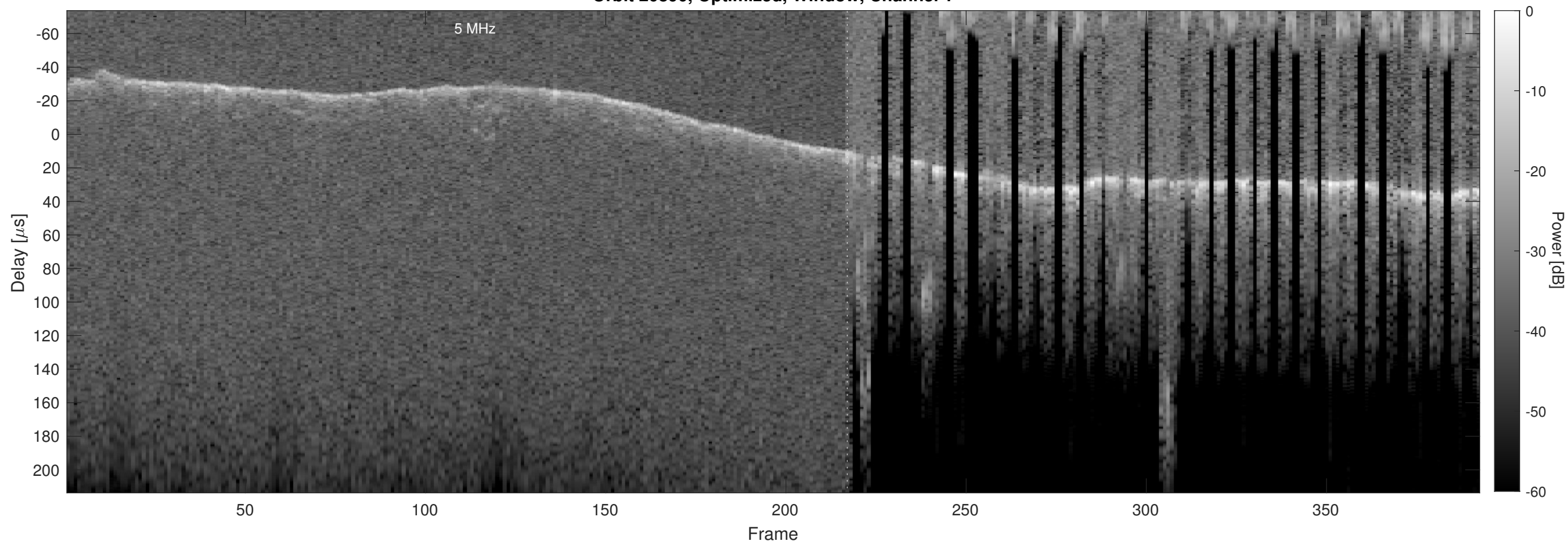
Orbit 20890, Optimized, Window, Channel 2
