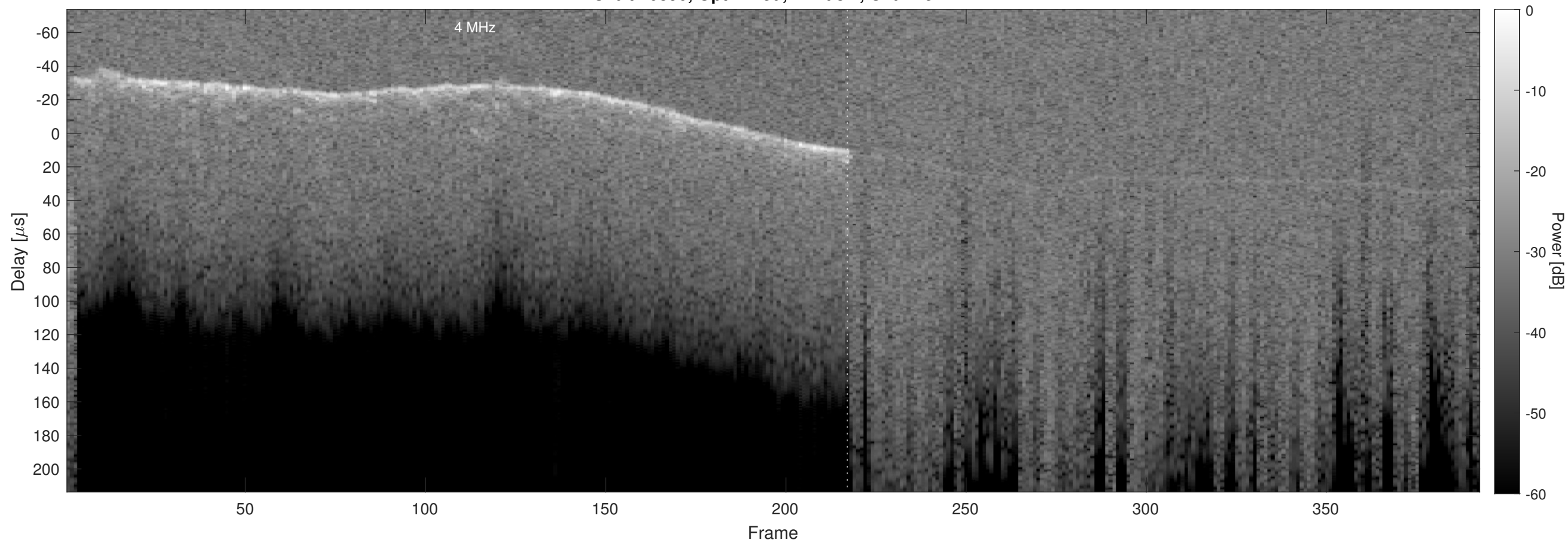
Orbit 20890, Optimized, Window, Channel 2
