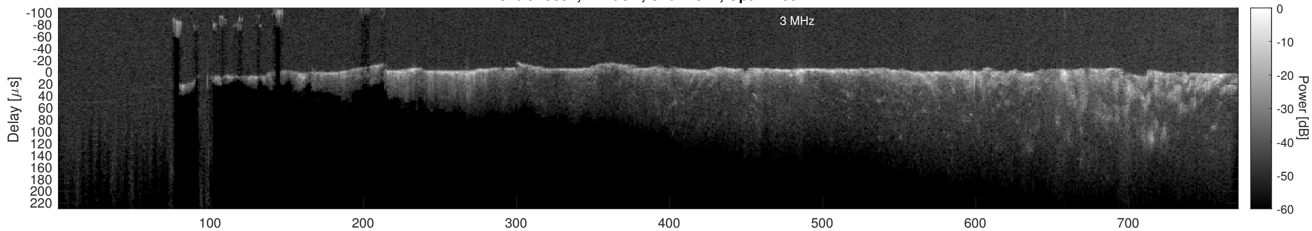
Orbit 20891, Cluttergram
