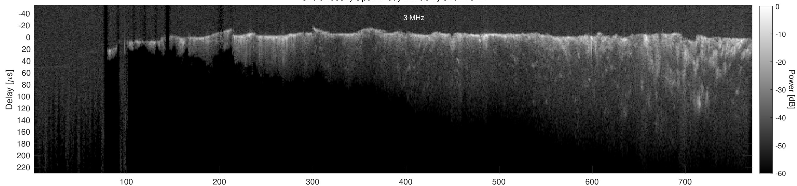
Orbit 20891, Cluttergram
