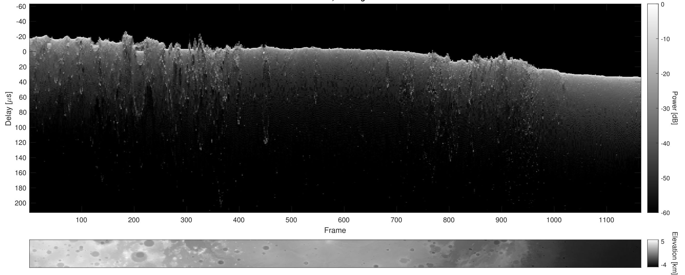
Orbit 20893, Cluttergram
