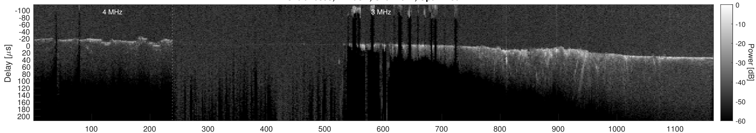
Orbit 20893, Cluttergram
