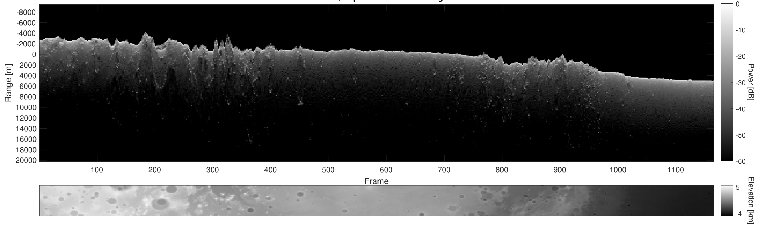
Orbit 20893, Depth-Corrected Cluttergram
