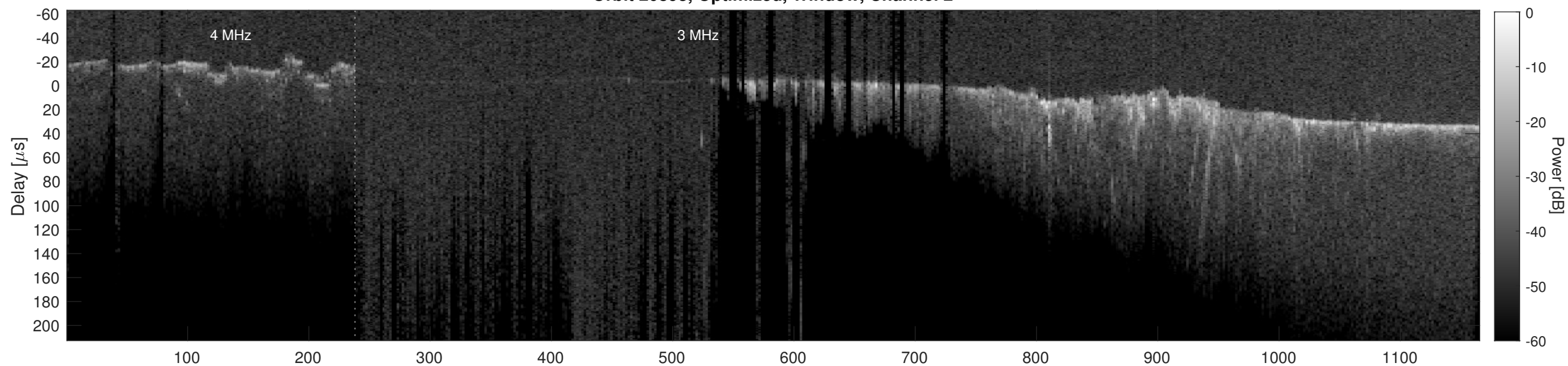
Orbit 20893, Cluttergram
