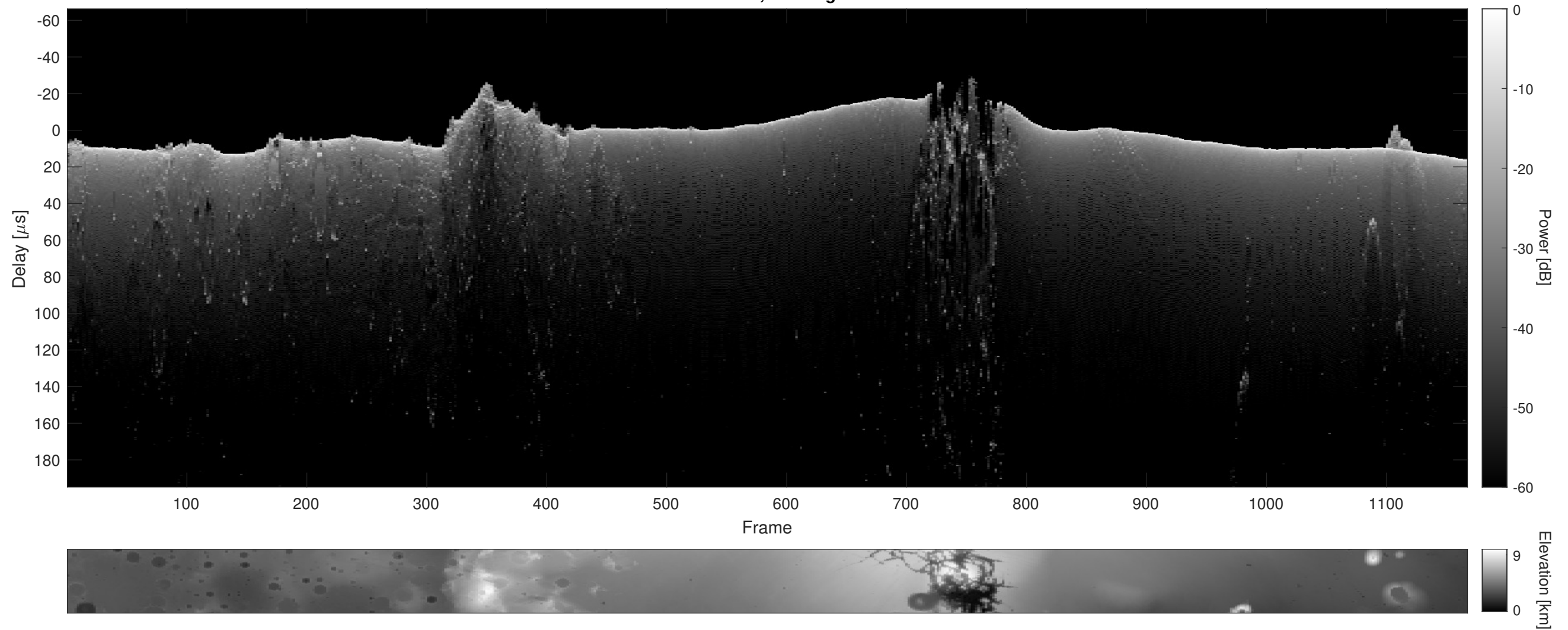
Orbit 20895, Cluttergram
