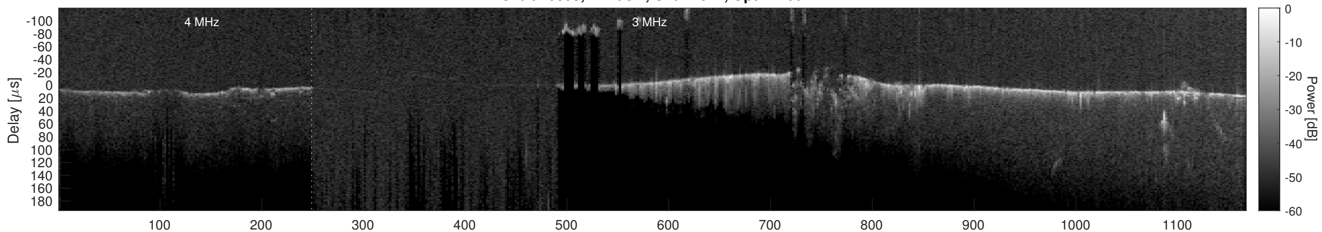
Orbit 20895, Cluttergram
