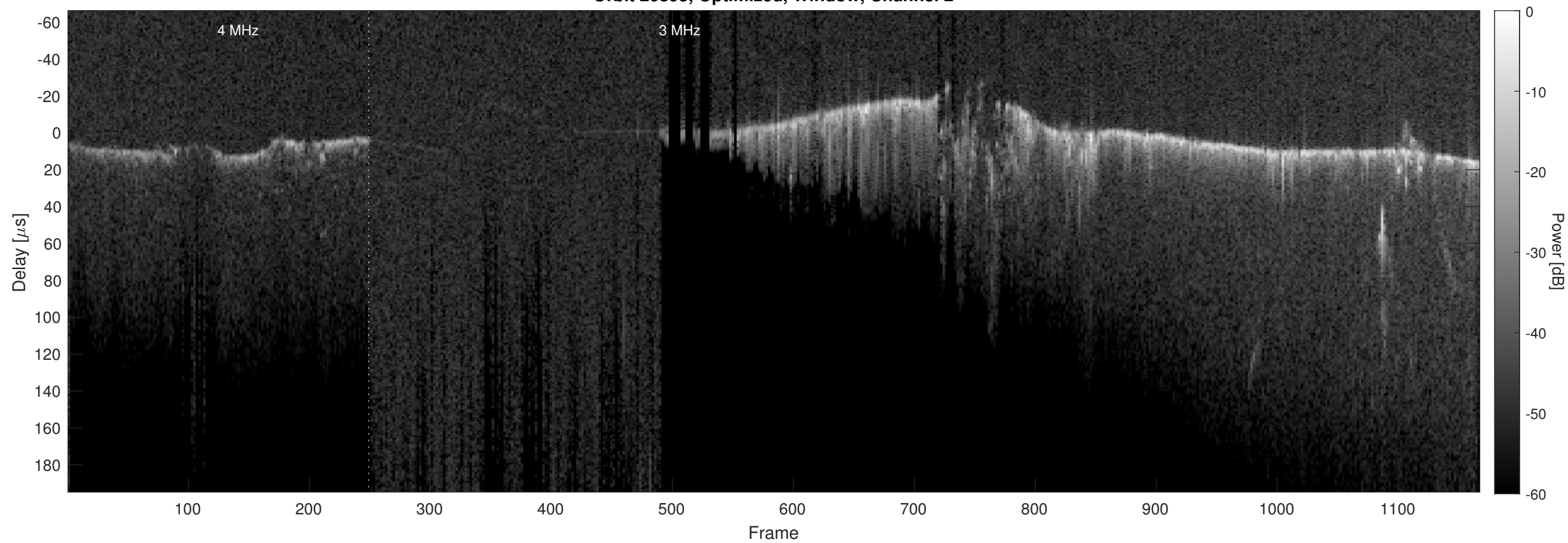
Orbit 20895, Optimized, Window, Channel 2
