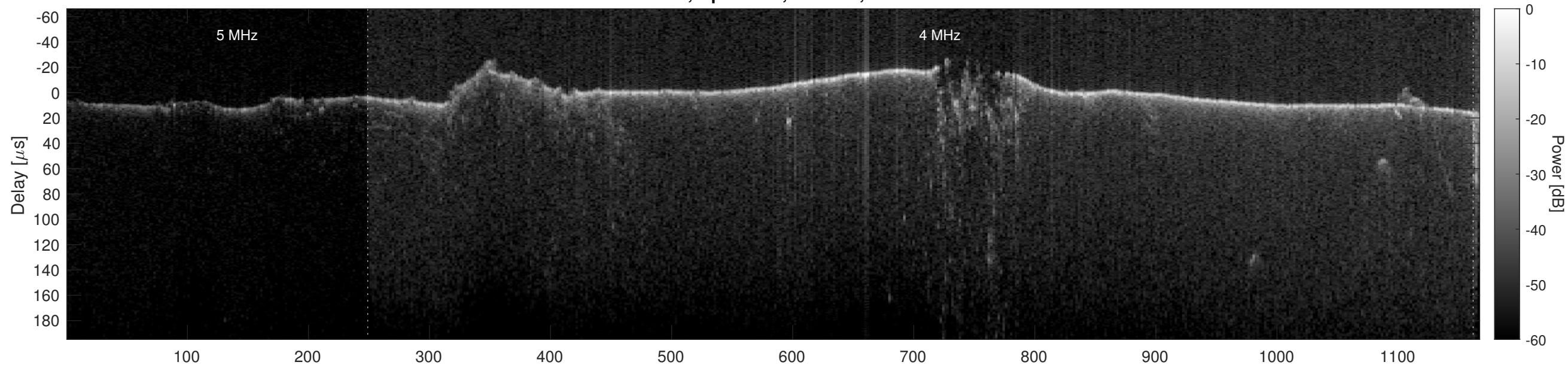
Orbit 20895, Optimized, Window, Channel 2
