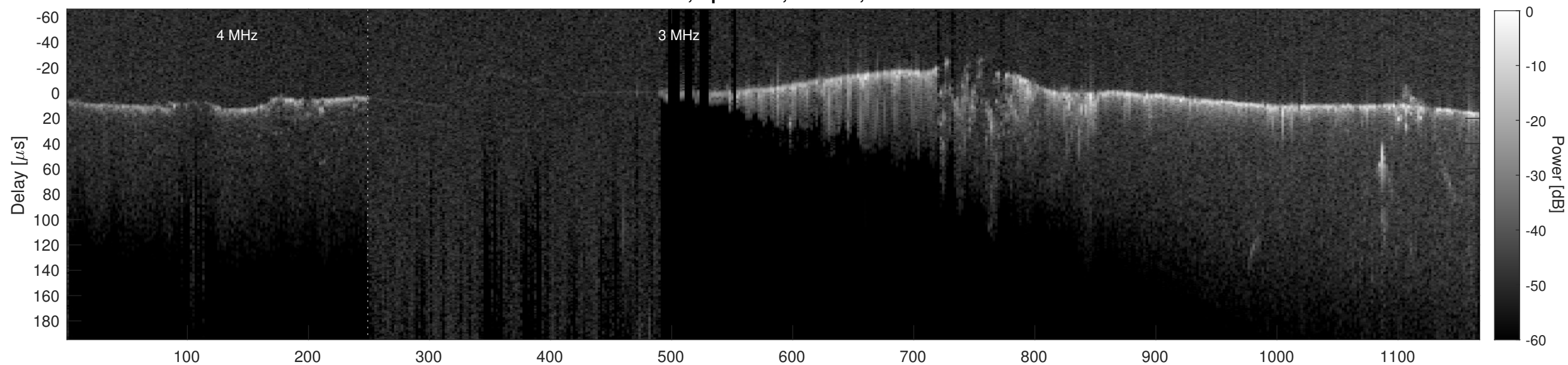
Orbit 20895, Cluttergram
