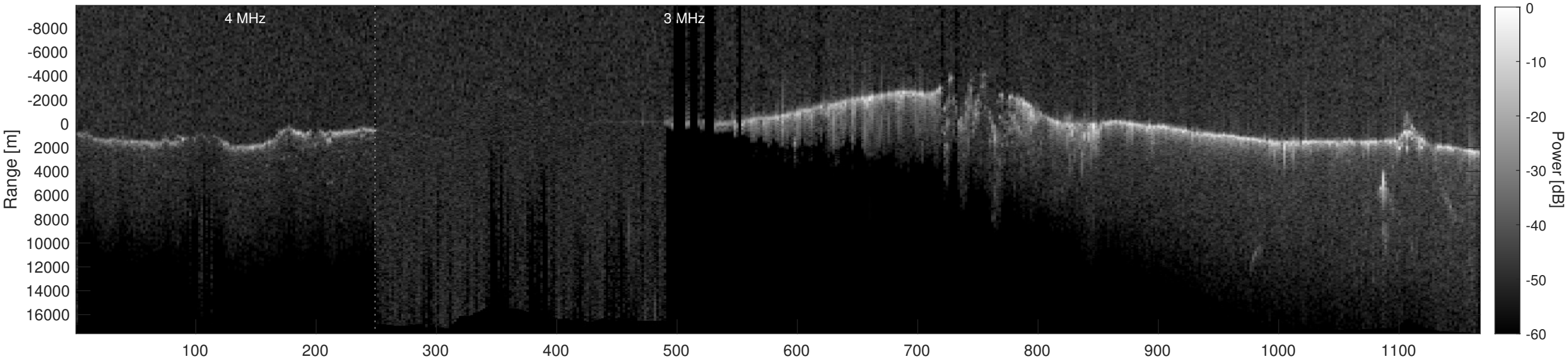
Orbit 20895, Depth-Corrected Cluttergram
