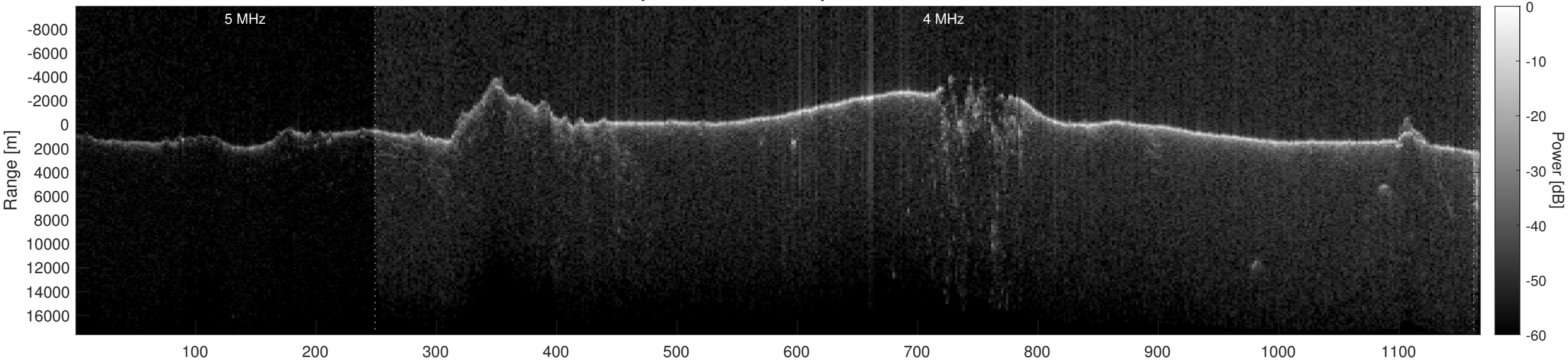
Orbit 20895, Optimized, Window, Depth-Corrected, Channel 2
