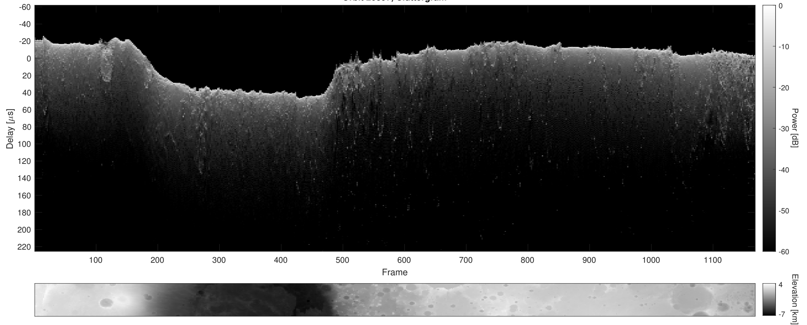
Orbit 20897, Cluttergram
