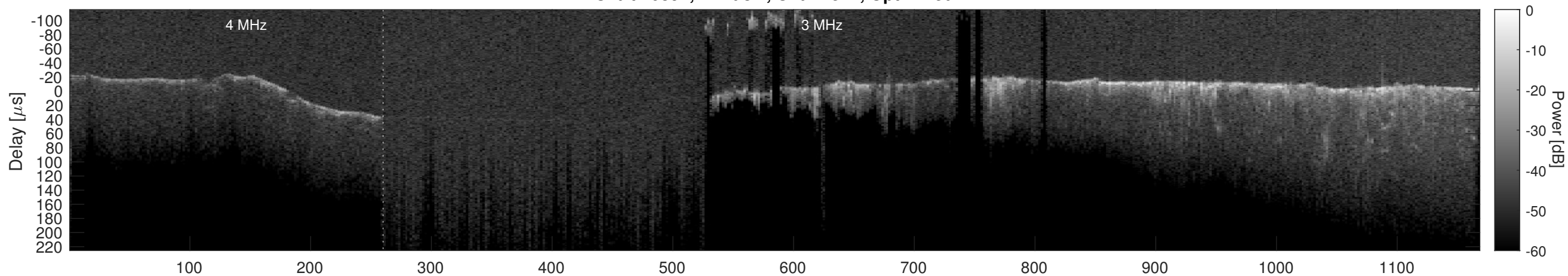
Orbit 20897, Cluttergram
