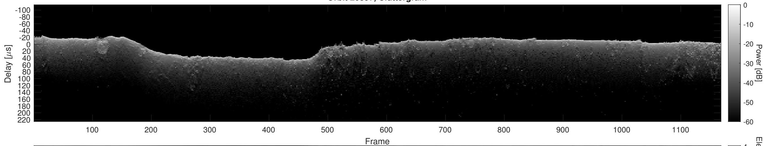
Orbit 20897, Cluttergram
