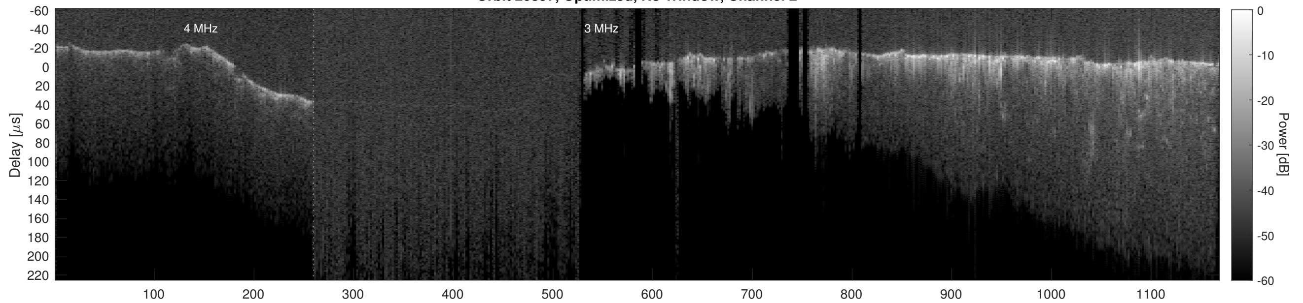
Orbit 20897, Cluttergram
