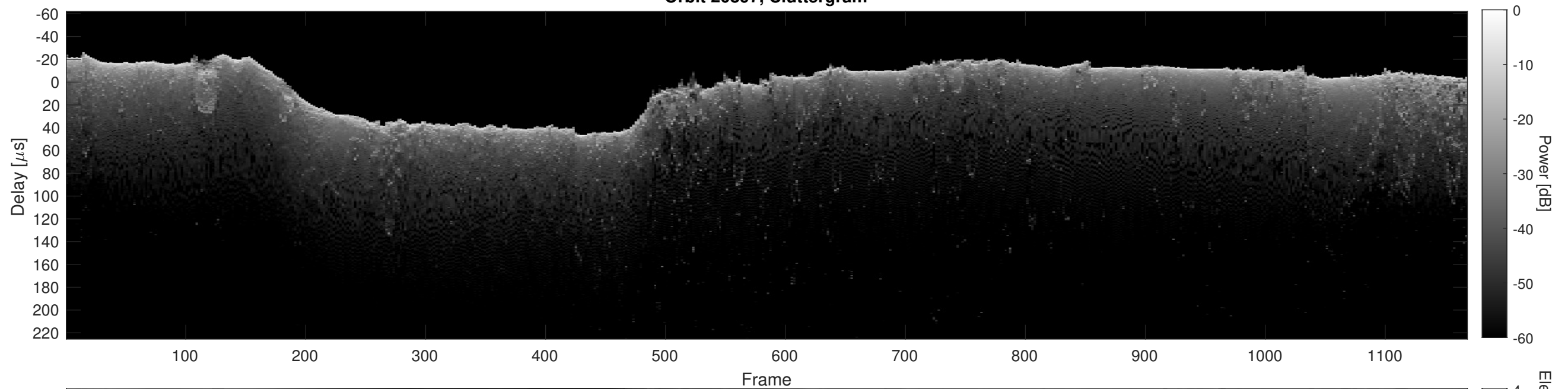
Orbit 20897, Cluttergram
