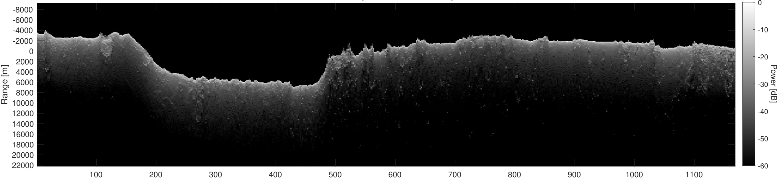
Orbit 20897, Depth-Corrected Cluttergram
