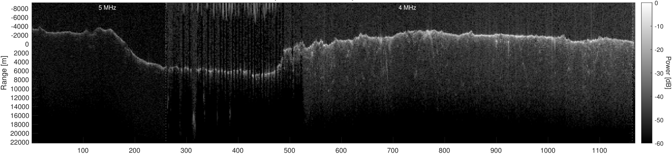
Orbit 20897, Optimized, Window, Depth-Corrected, Channel 2
