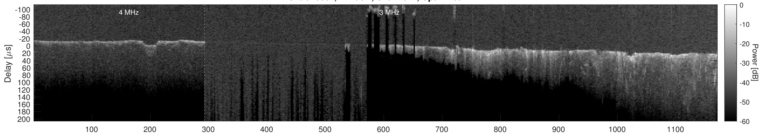
Orbit 20901, Cluttergram
