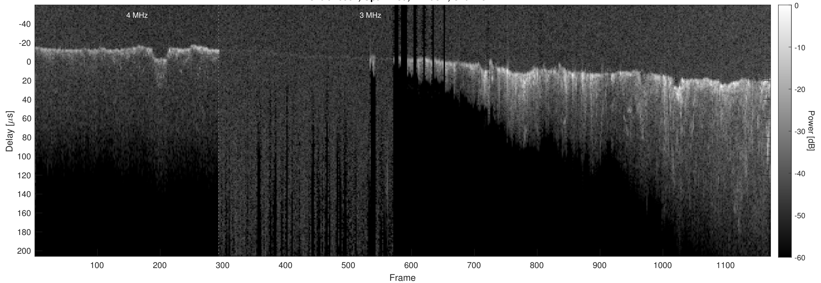
Orbit 20901, Optimized, Window, Channel 2
