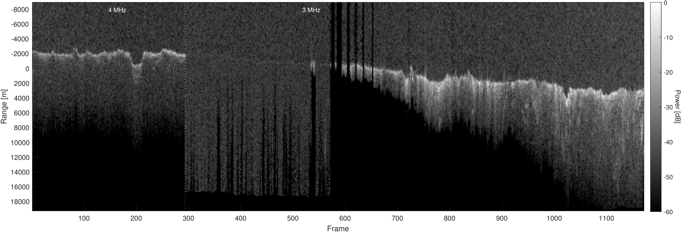
Orbit 20901, Optimized, Window, Depth-Corrected, Channel 2
