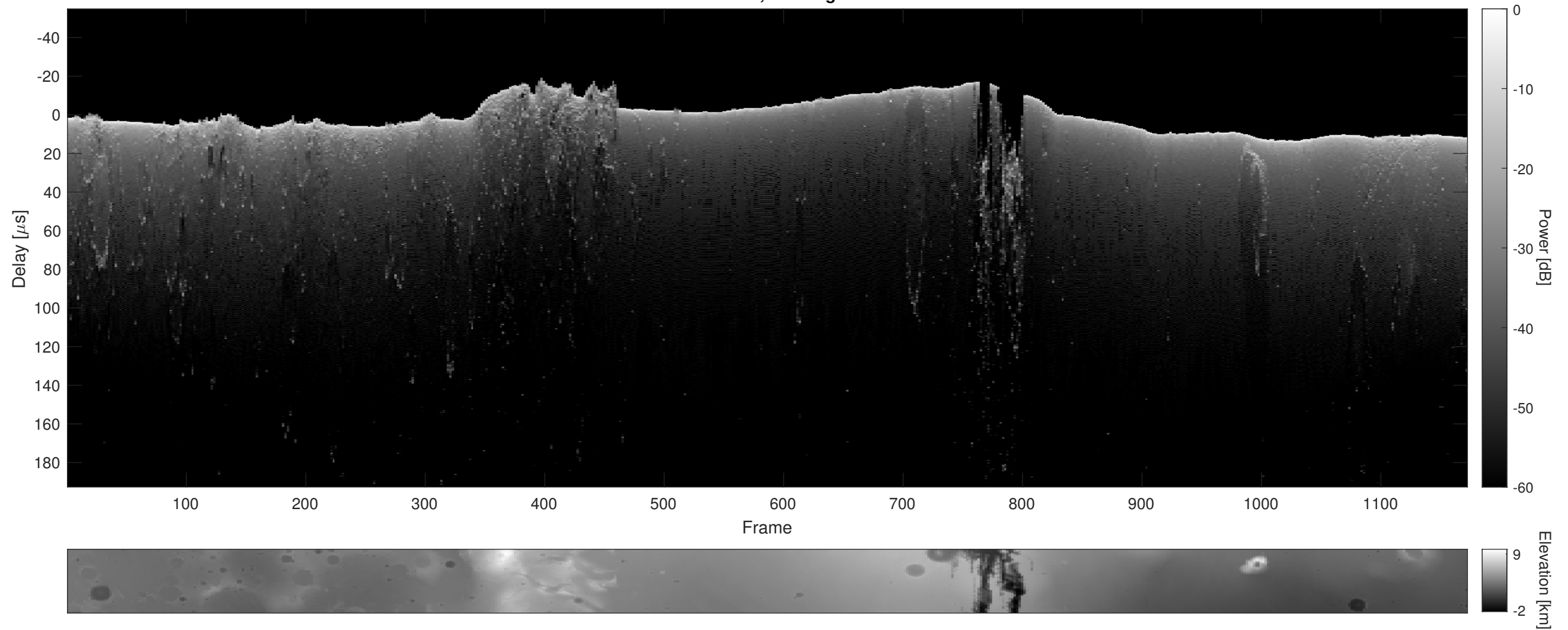
Orbit 20902, Cluttergram
