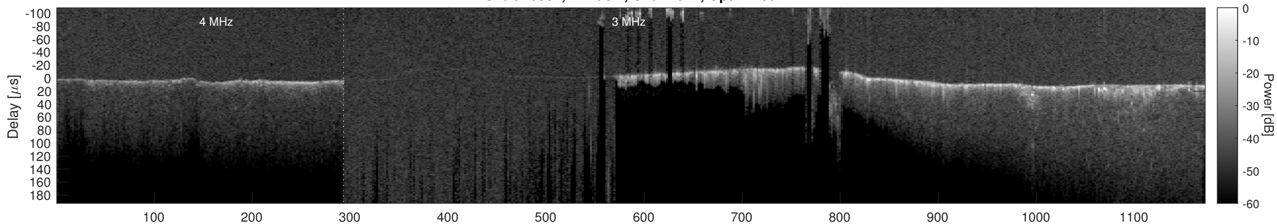
Orbit 20902, Cluttergram
