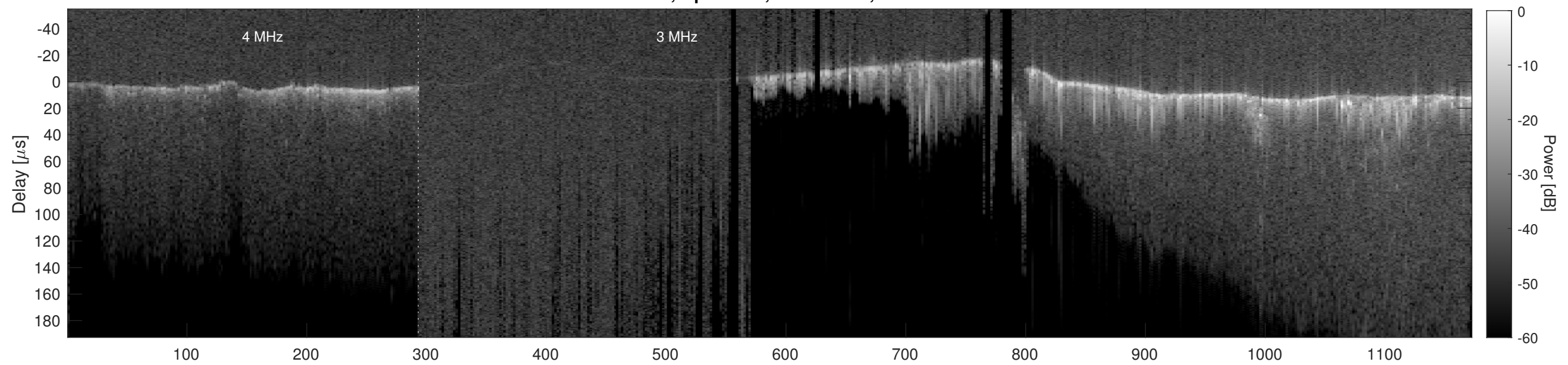
Orbit 20902, Cluttergram
