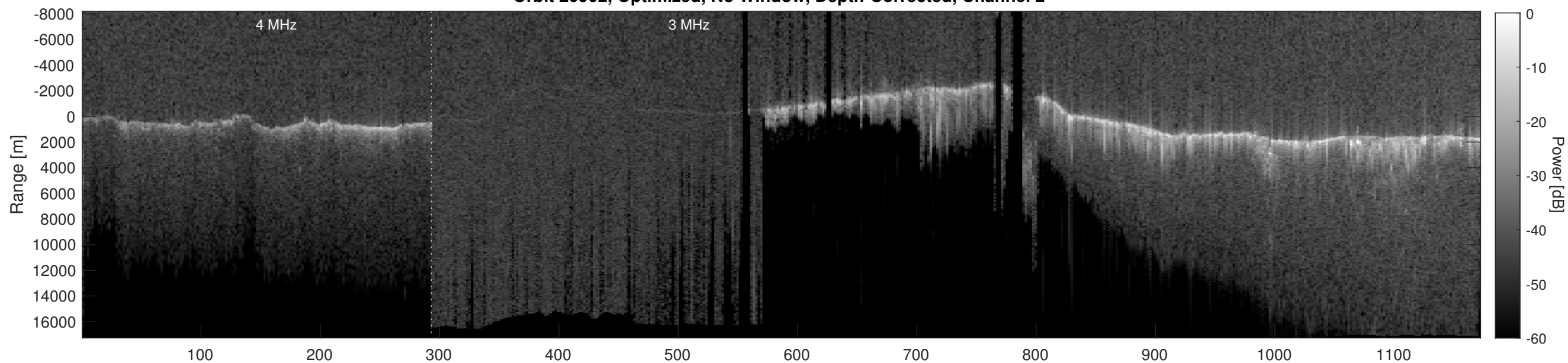
Orbit 20902, Depth-Corrected Cluttergram
