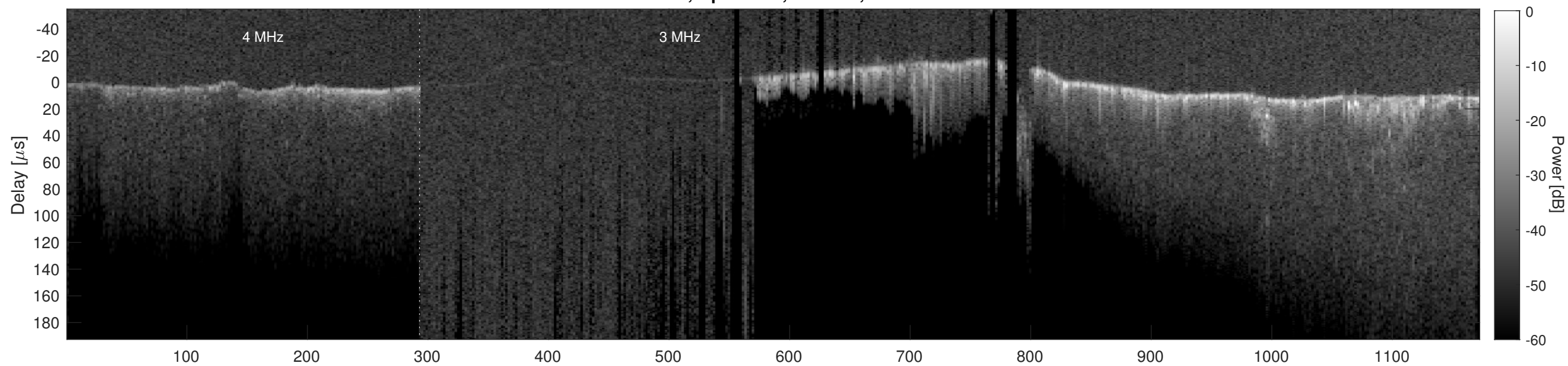
Orbit 20902, Cluttergram
