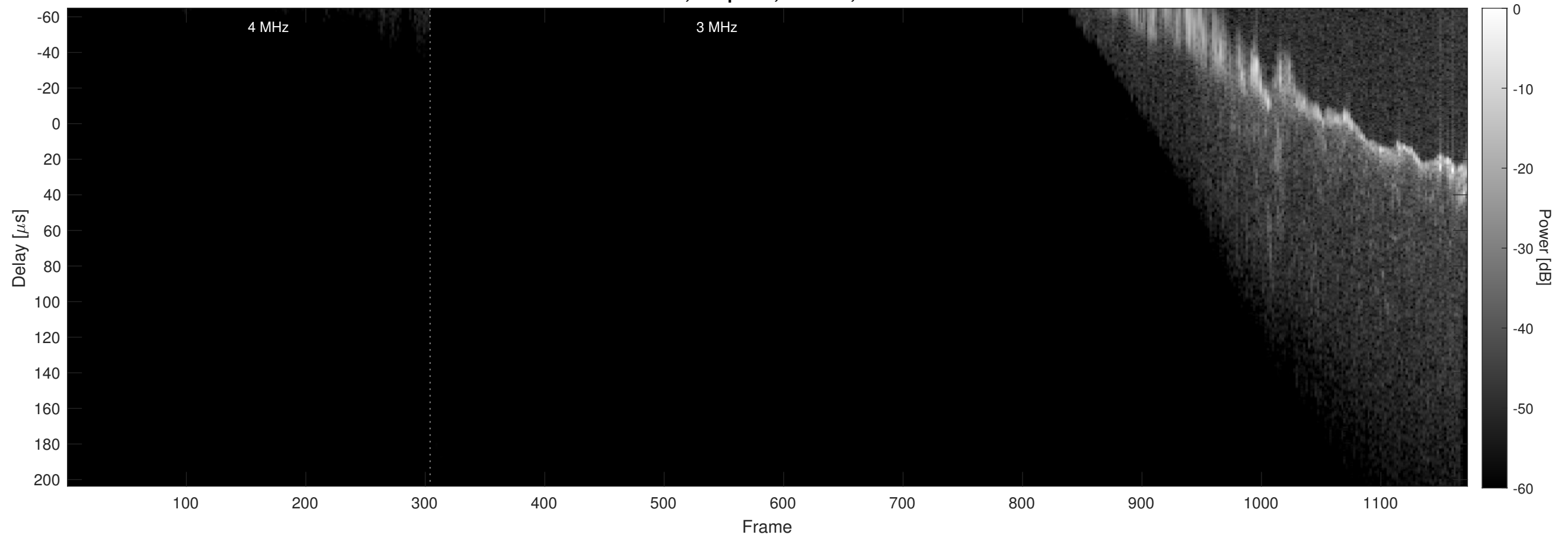
Orbit 20903, Chapman, Window, Channel 2
