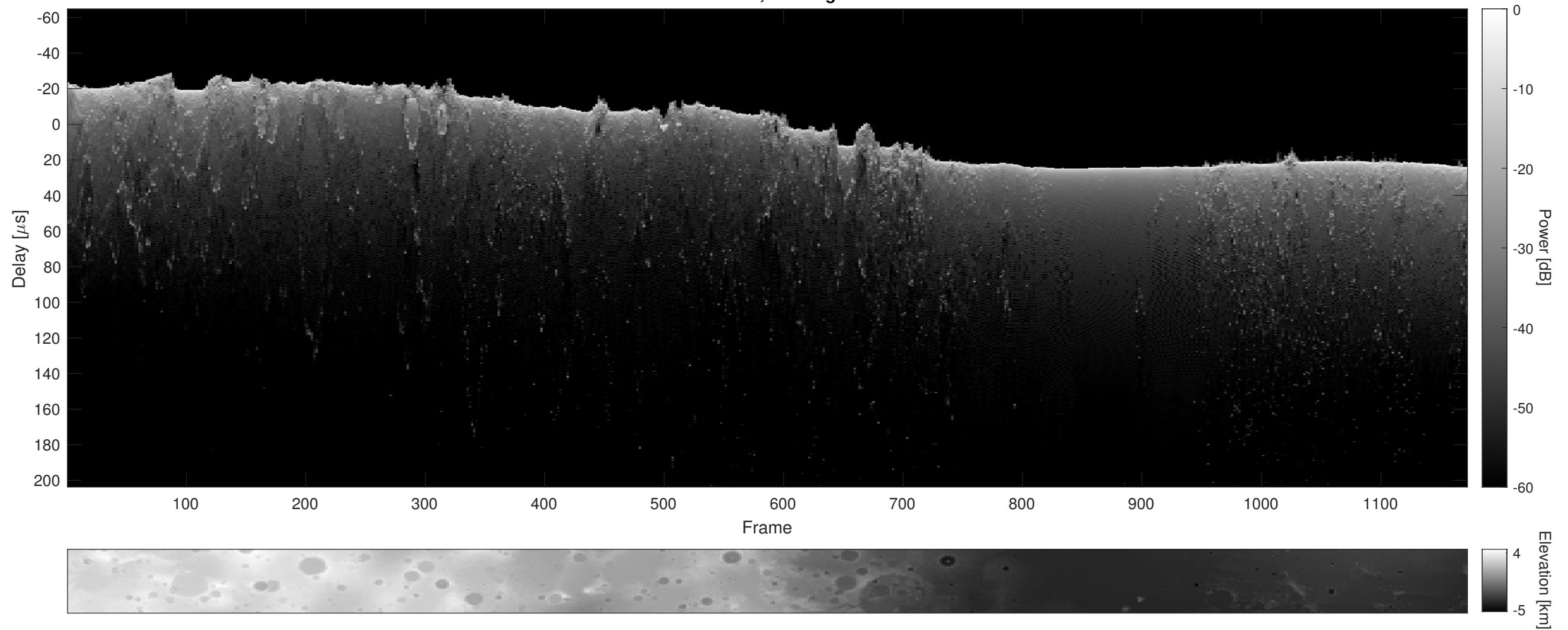
Orbit 20903, Cluttergram
