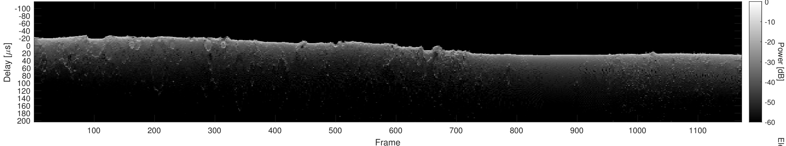
Orbit 20903, Cluttergram
