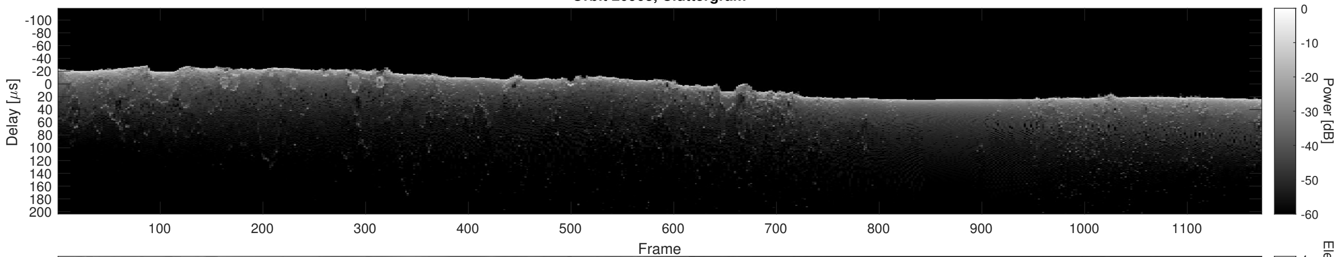
Orbit 20903, Cluttergram
