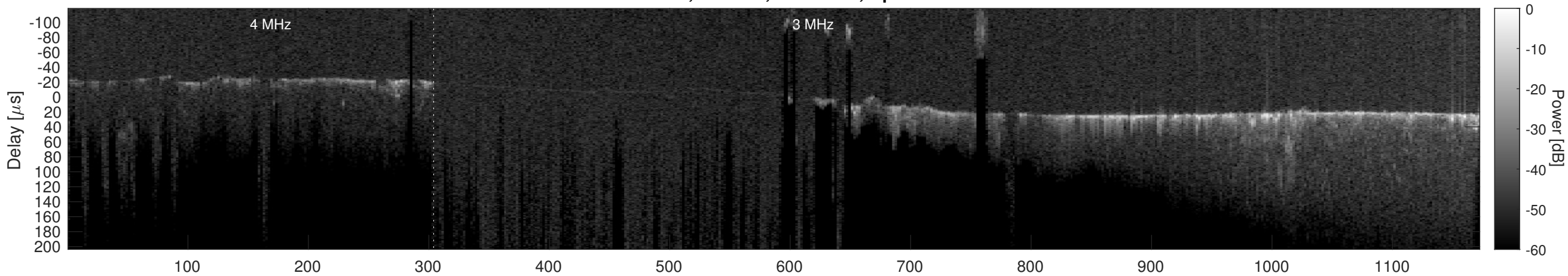
Orbit 20903, Cluttergram
