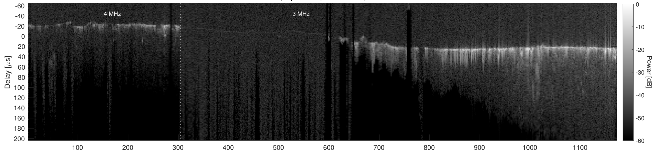
Orbit 20903, Cluttergram
