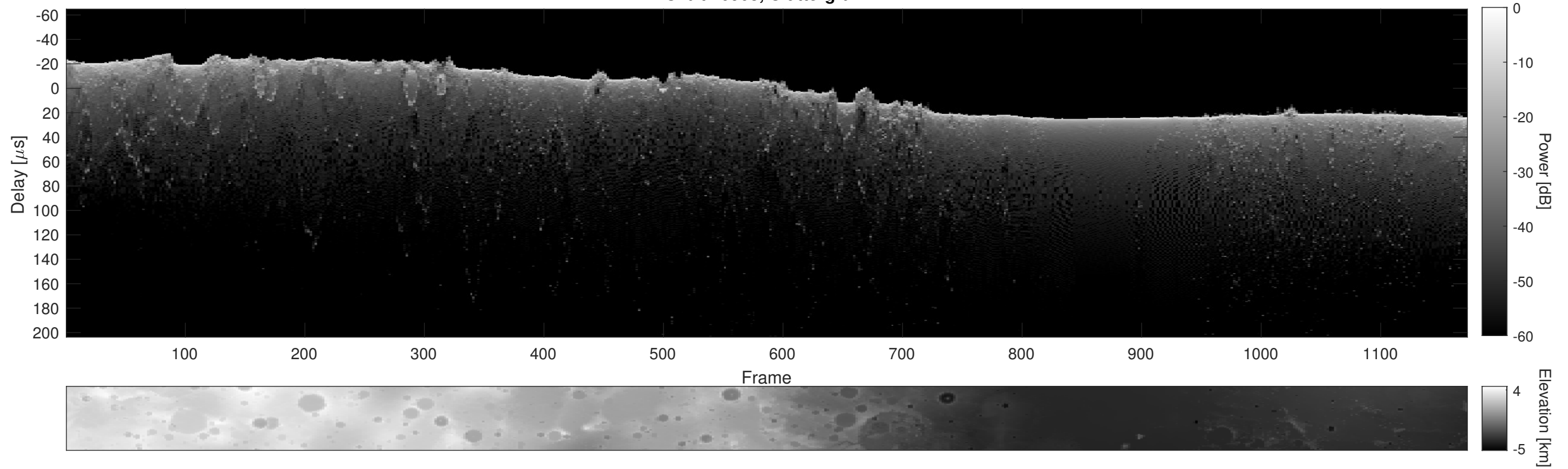
Orbit 20903, Cluttergram
