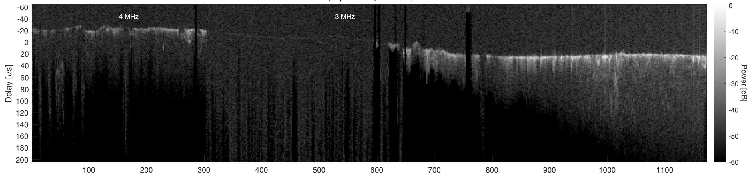
Orbit 20903, Cluttergram
