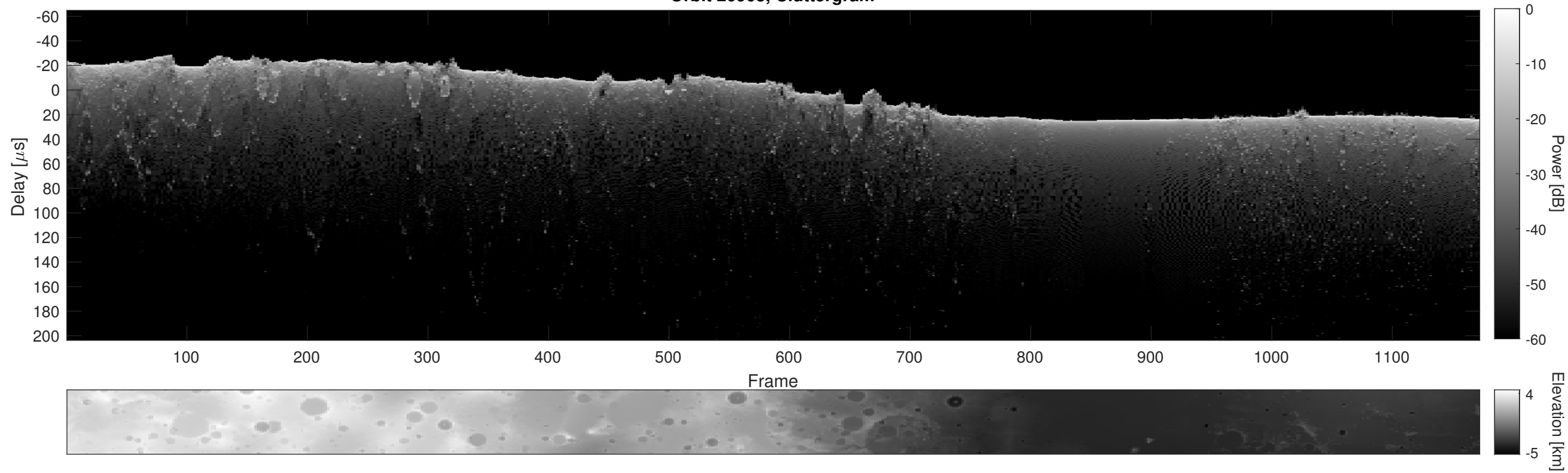
Orbit 20903, Cluttergram
