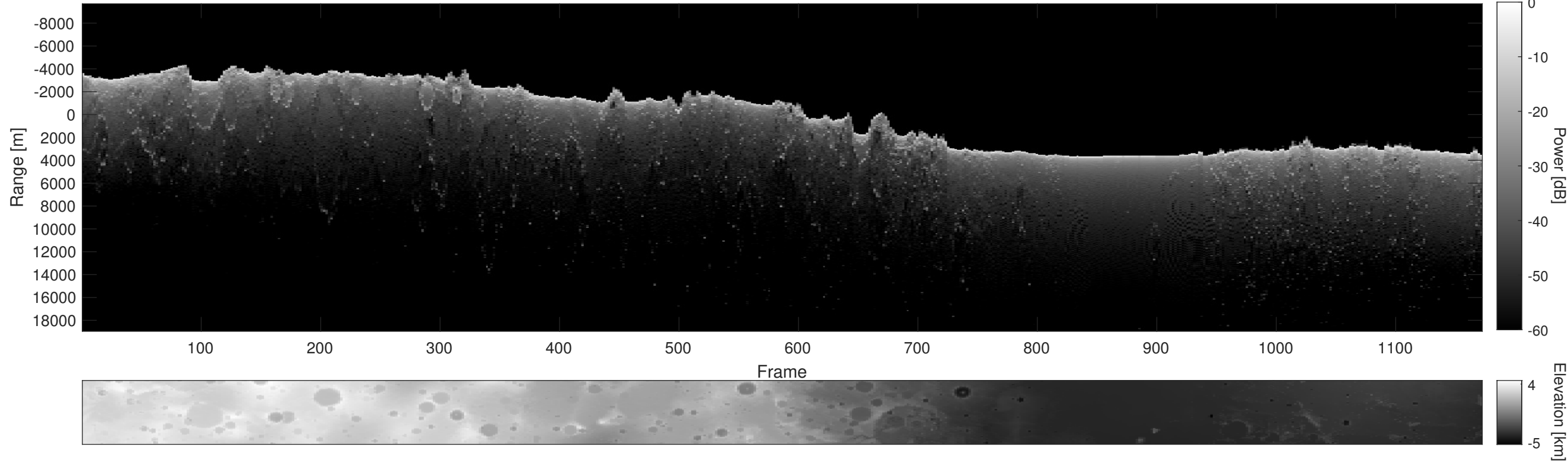
Orbit 20903, Depth-Corrected Cluttergram
