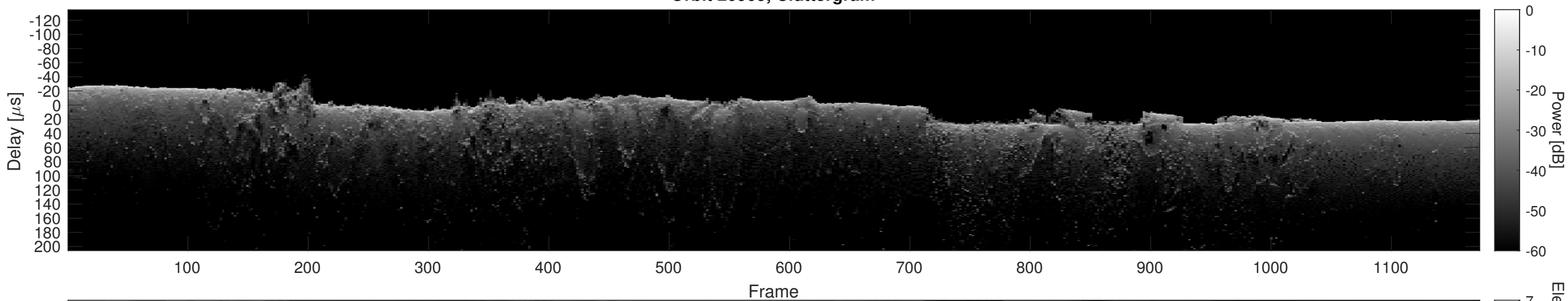
Orbit 20905, Cluttergram
