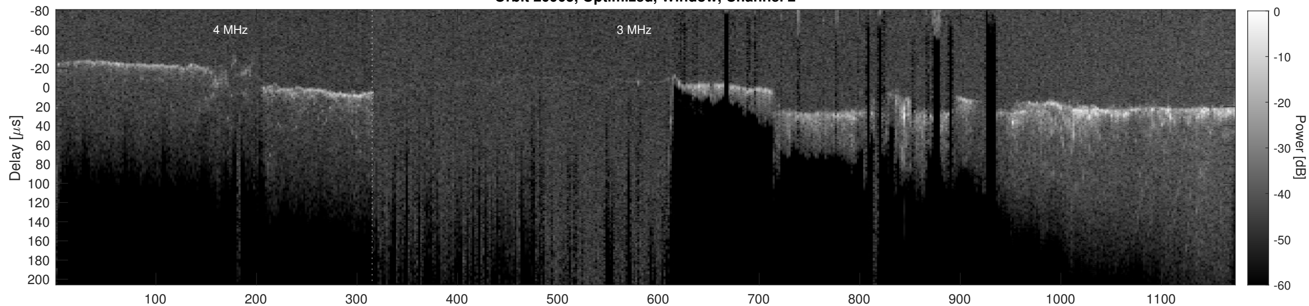
Orbit 20905, Cluttergram
