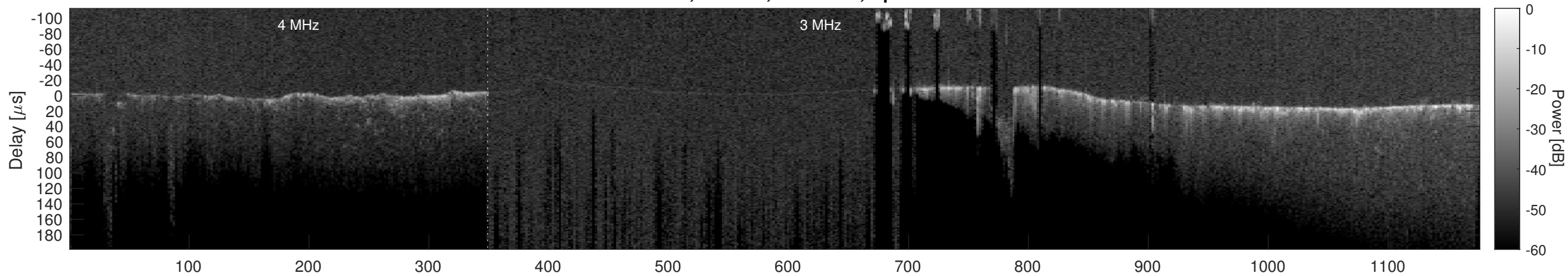
Orbit 20909, Cluttergram
