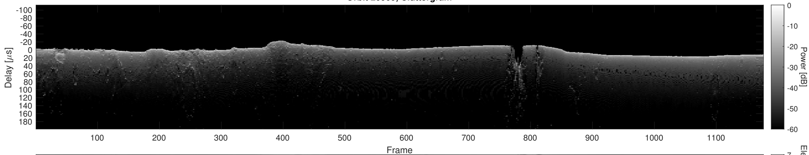
Orbit 20909, Cluttergram
