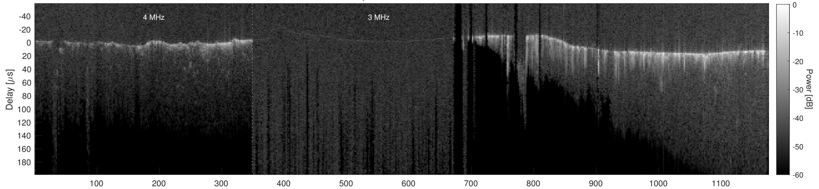
Orbit 20909, Cluttergram
