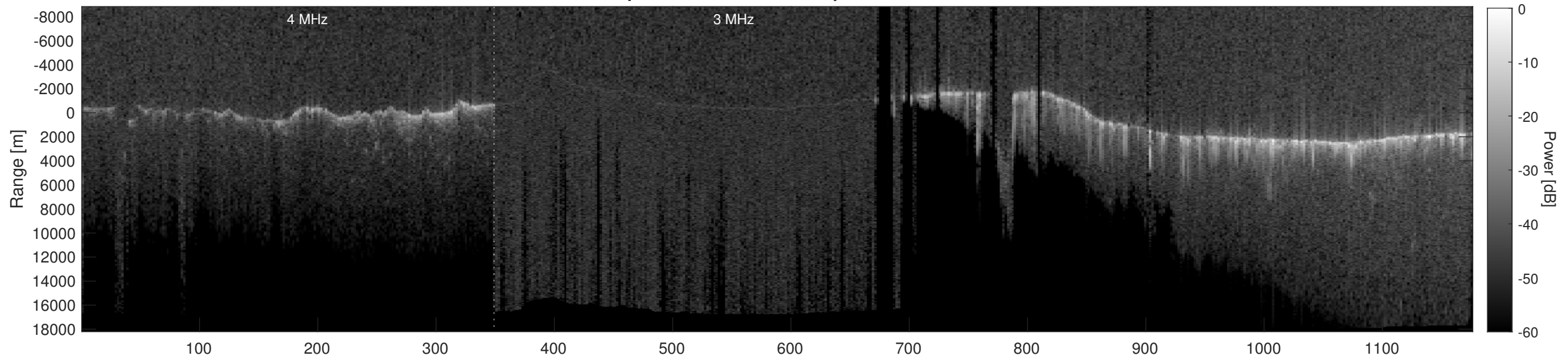
Orbit 20909, Depth-Corrected Cluttergram
