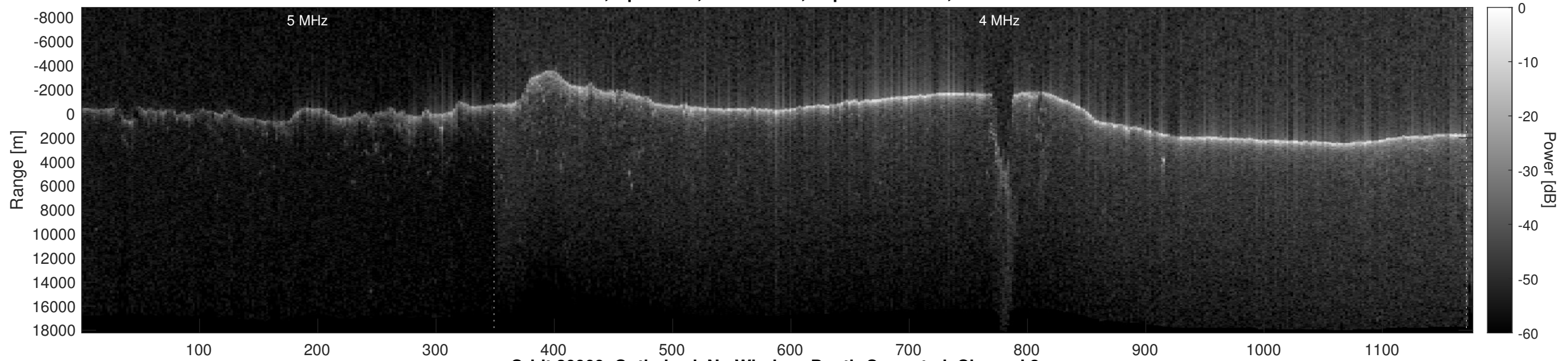
Orbit 20909, Optimized, No Window, Depth-Corrected, Channel 2
