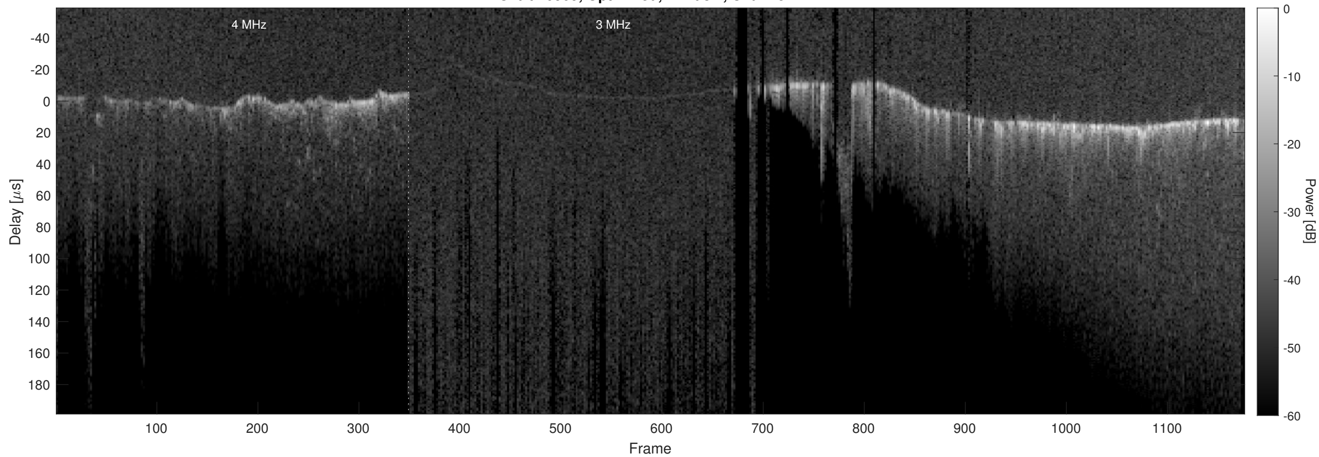
Orbit 20909, Optimized, Window, Channel 2
