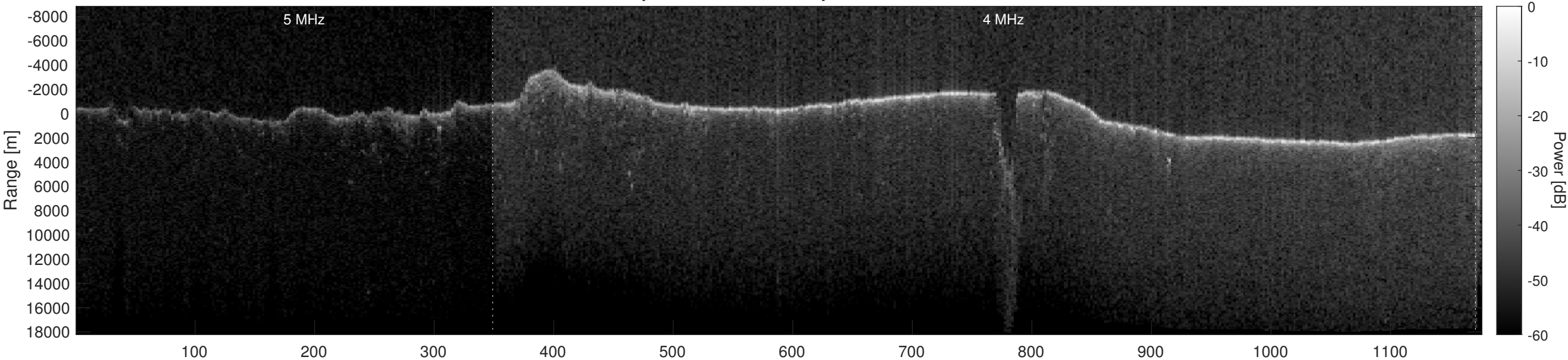
Orbit 20909, Optimized, Window, Depth-Corrected, Channel 2
