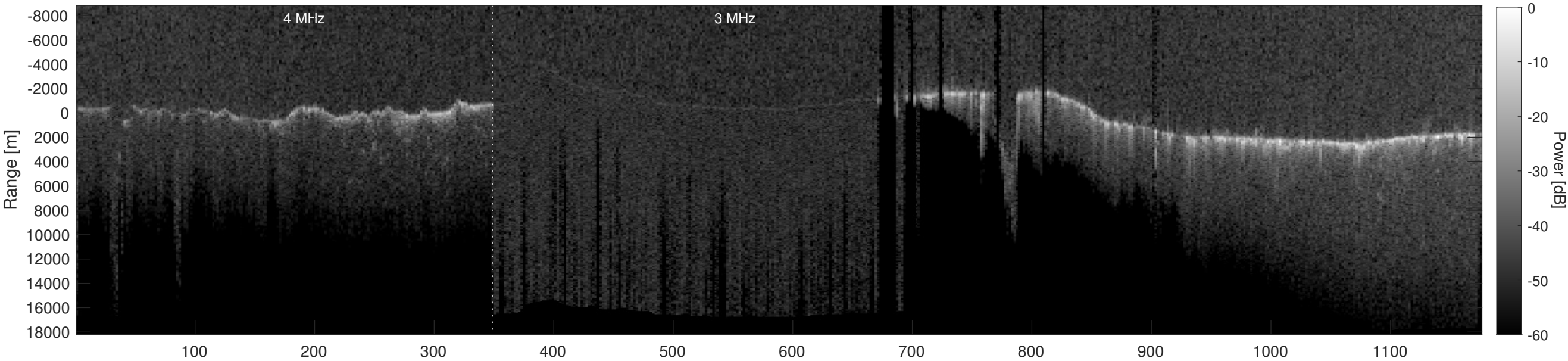
Orbit 20909, Depth-Corrected Cluttergram
