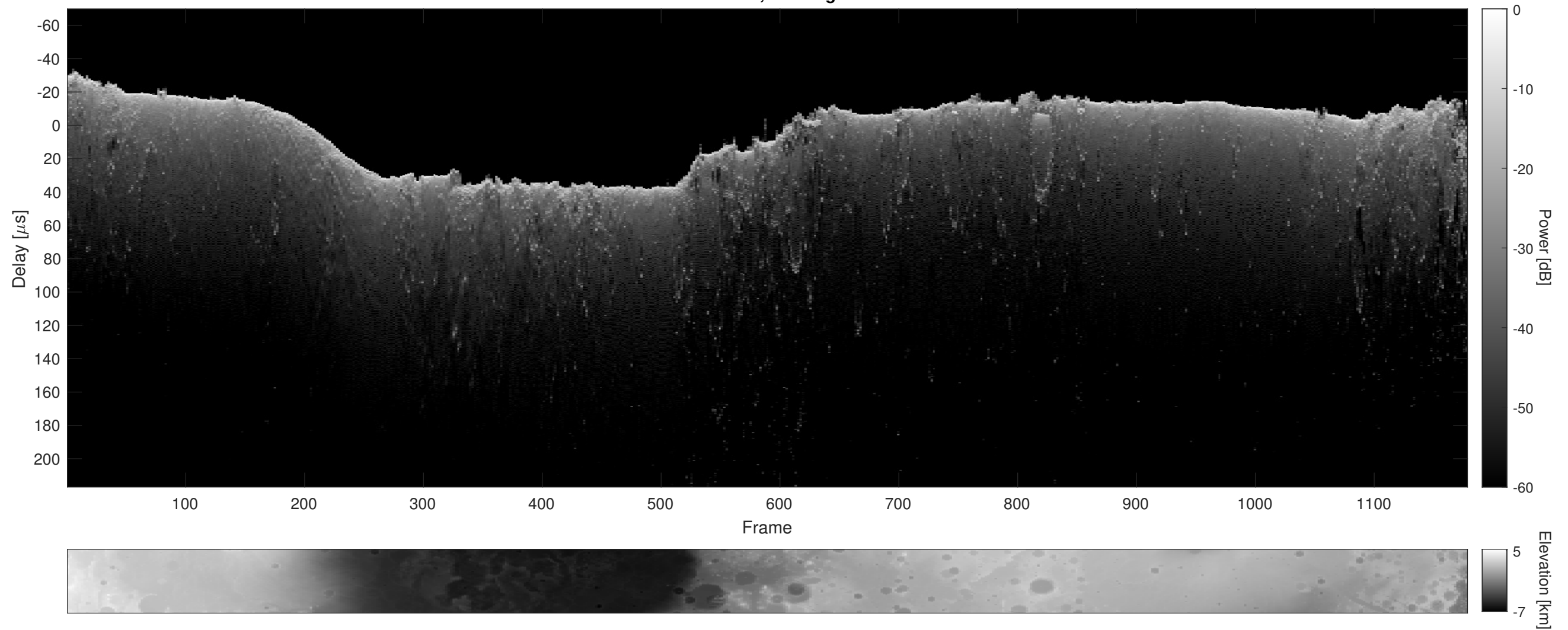
Orbit 20911, Cluttergram
