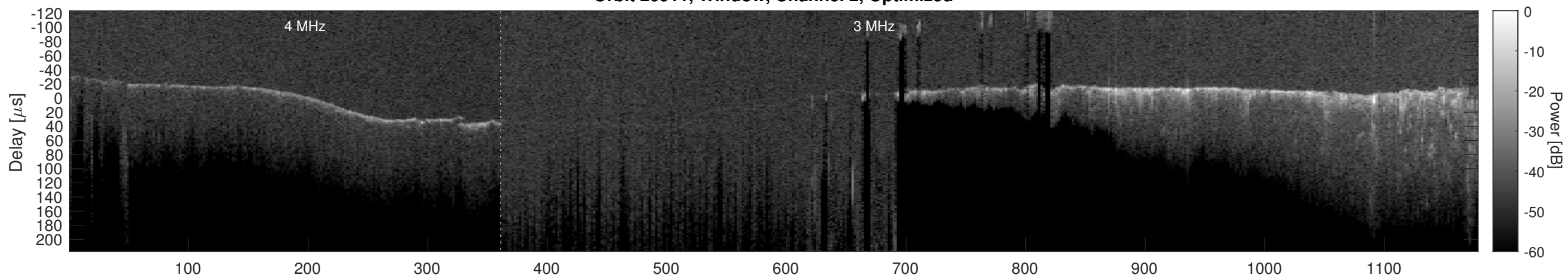
Orbit 20911, Cluttergram
