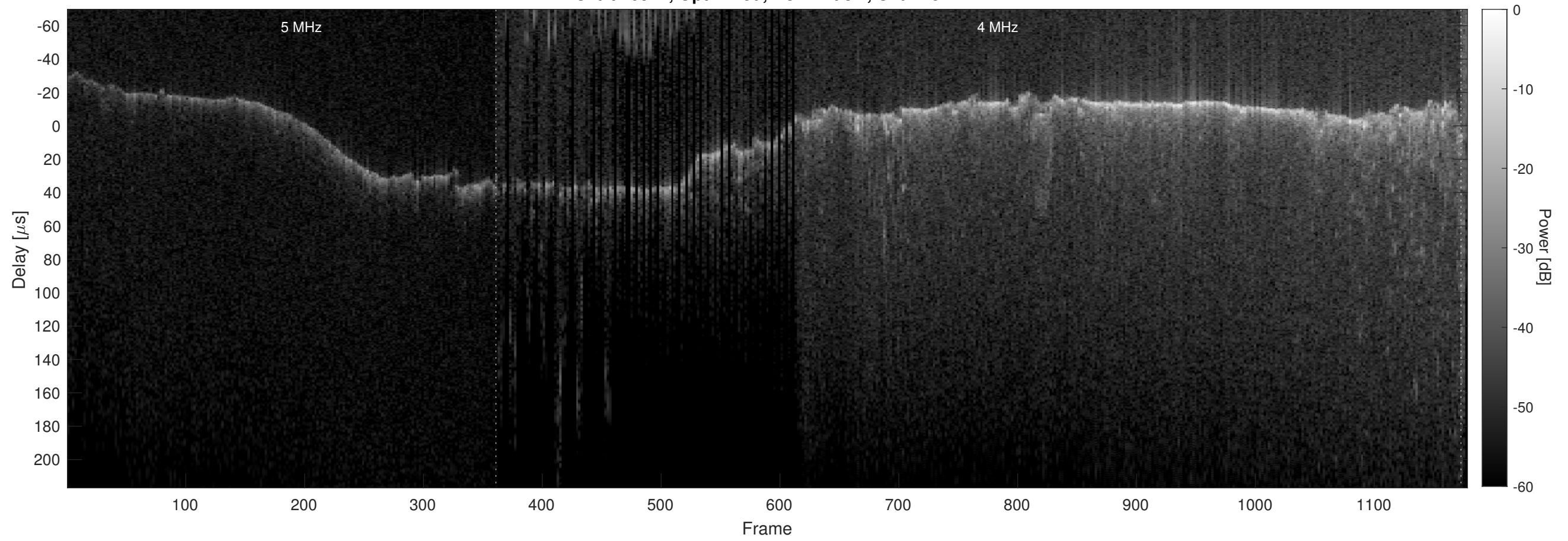
Orbit 20911, Optimized, No Window, Channel 2
