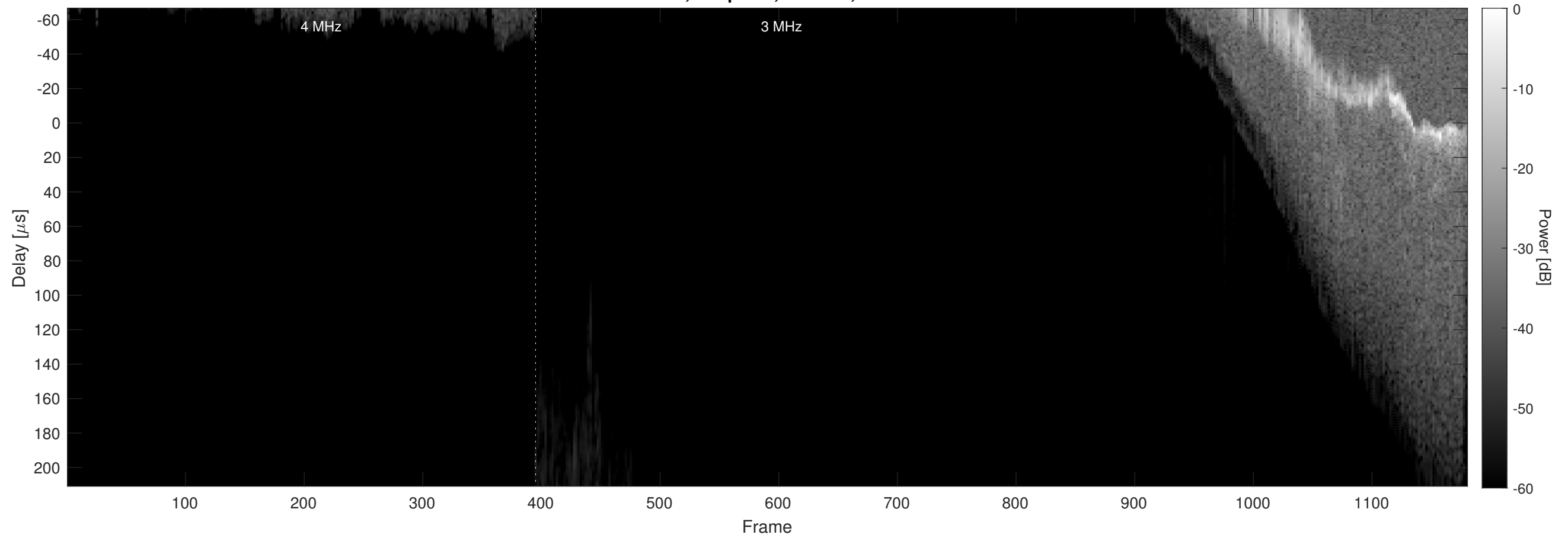
Orbit 20916, Chapman, Window, Channel 2
