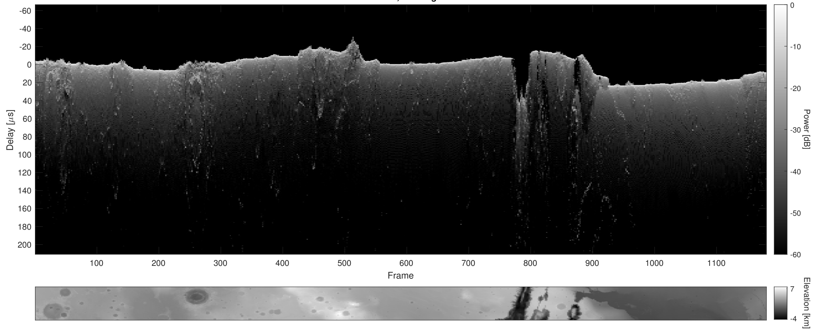
Orbit 20916, Cluttergram
