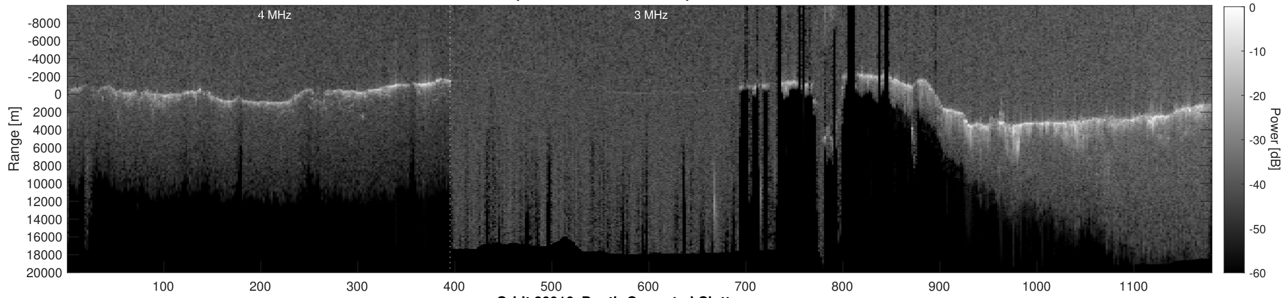
Orbit 20916, Depth-Corrected Cluttergram
