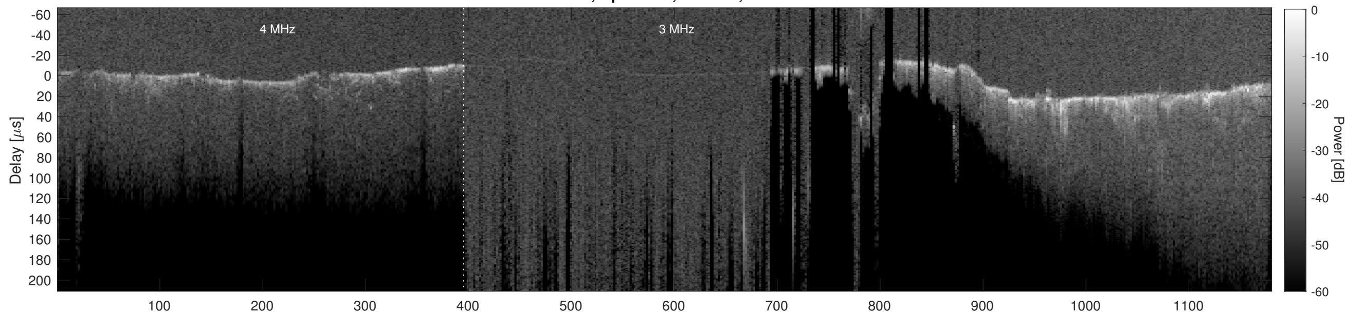
Orbit 20916, Cluttergram
