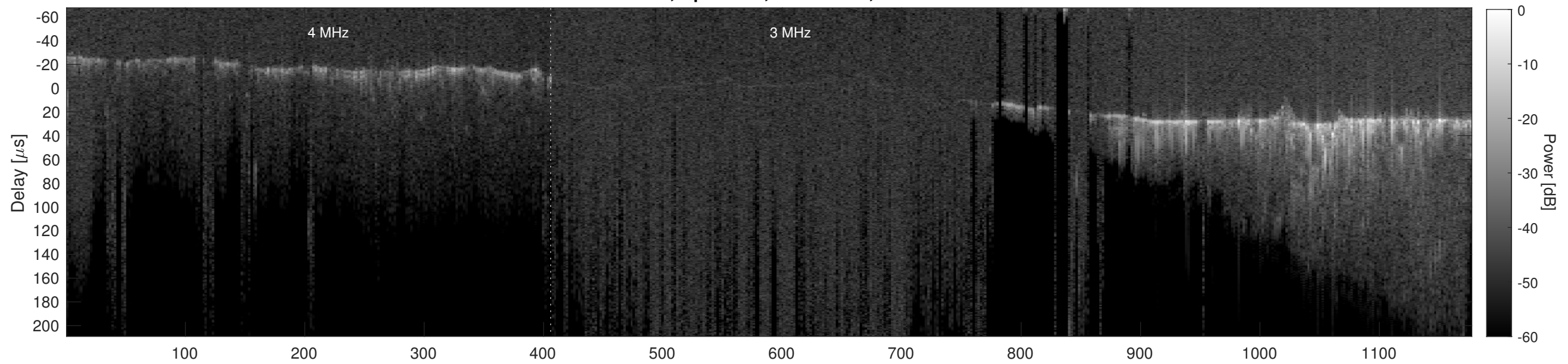
Orbit 20917, Cluttergram
