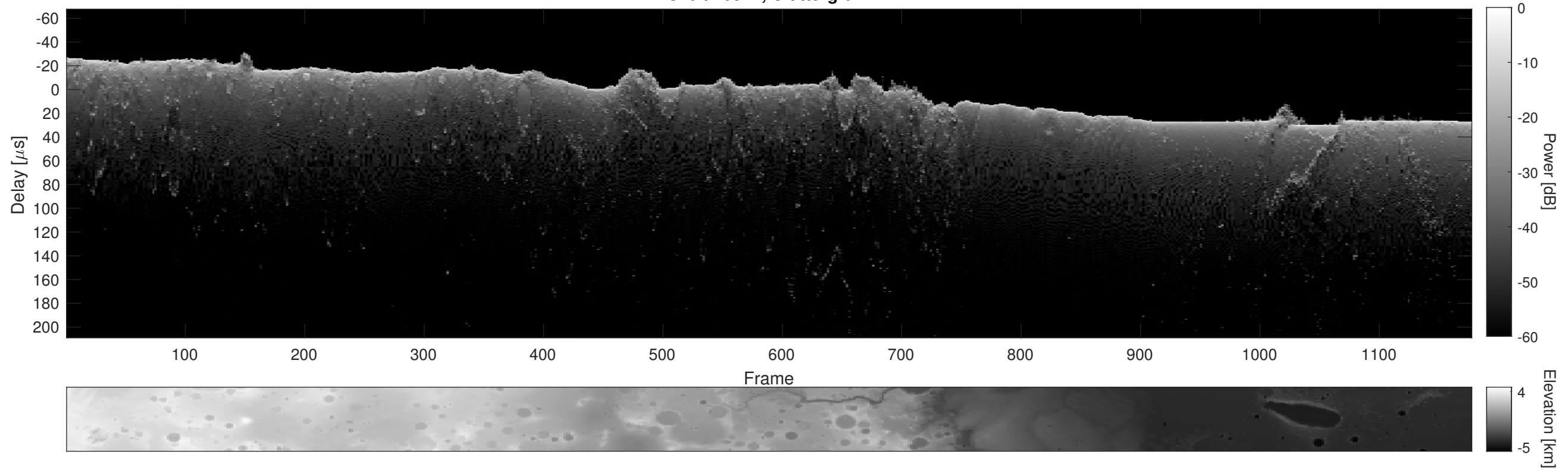
Orbit 20917, Cluttergram
